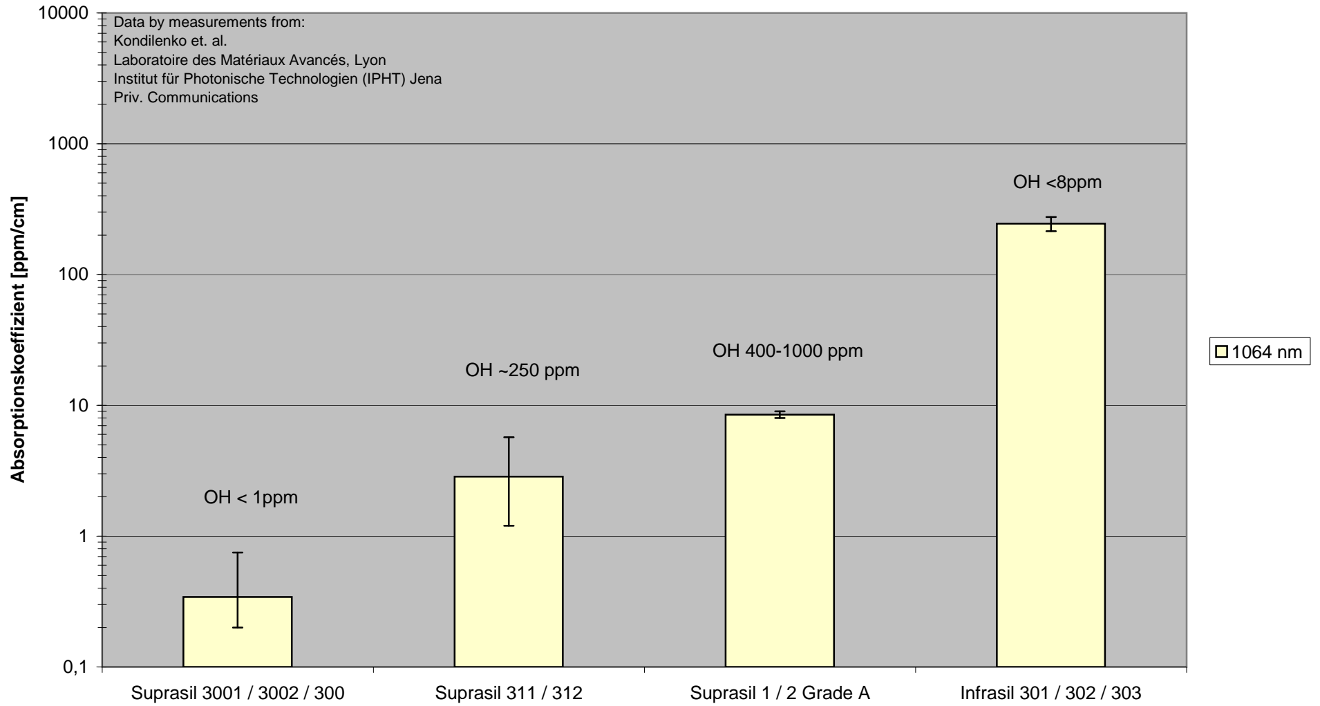
Typical Absorption of different Heraeus Material Grades @ Wavelength = 1064nm
